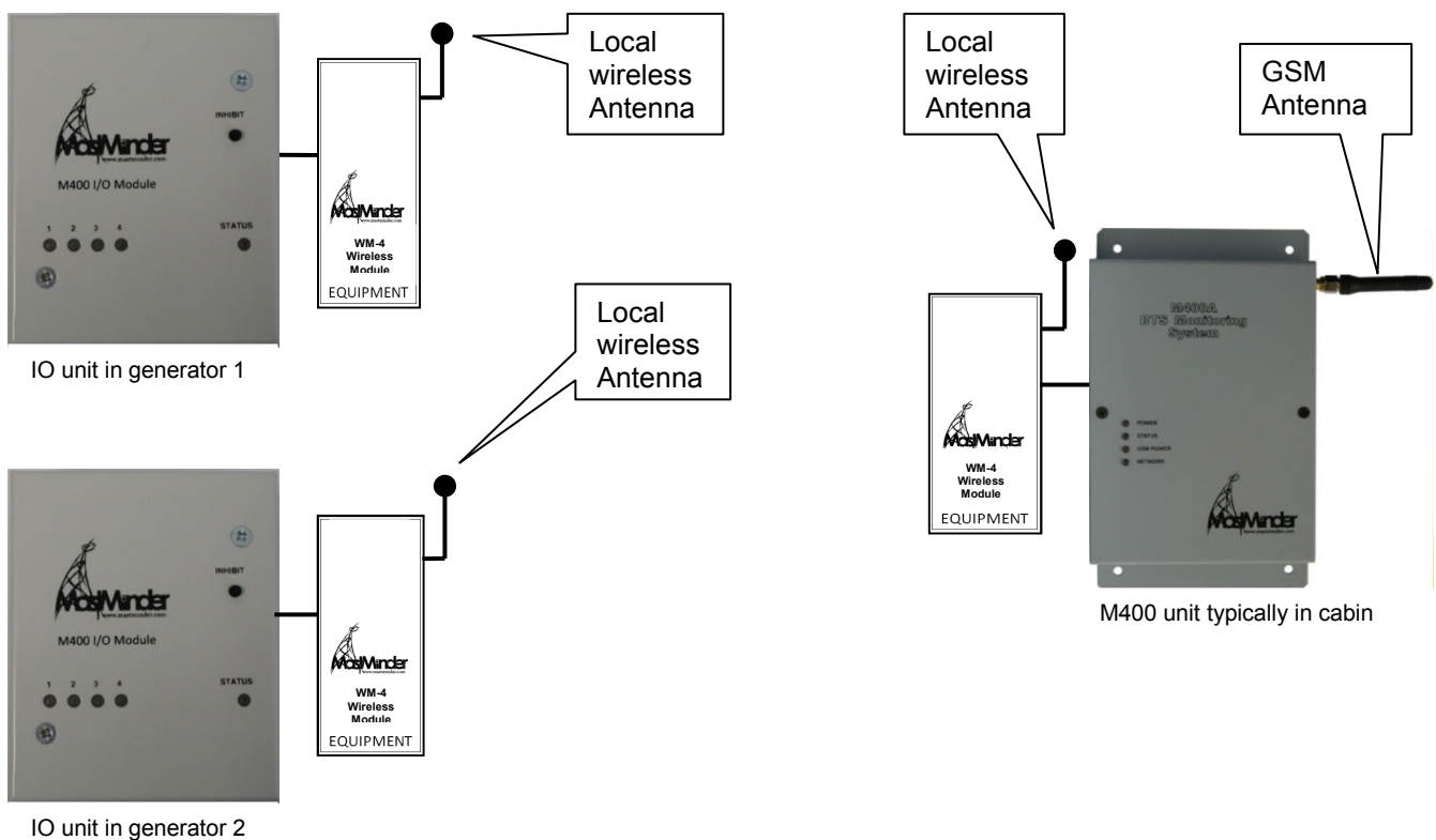
Typical Installation
